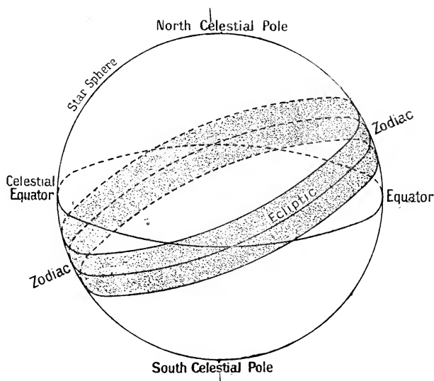
Fig. 4. The star sphere.
